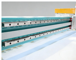
高精直线导轨, 保证机头、鞍架高速运行平稳 High precision linear guide rails ensure the sewing head and saddle running smoothly at a high speed
